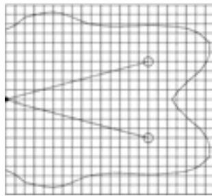
2 x 20W Flood Unit
