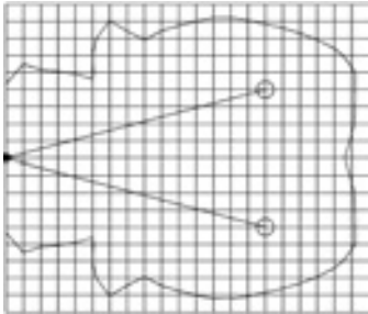
2 x 12W Flood Unit
